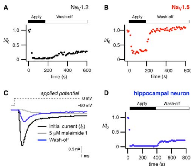
Figure 2. Representative time courses of wash-off of 5 \mu\text{M} 1 from CHO cells expressing rNa v 1.2 (A) and hNa v 1.5 (B). Average current recovery after washout was 25 \pm 1\% of I_0 on rNa v 1.2, compared to 100 \pm 3\% on hNa v 1.5. (C) Current recordings, elicited by a 10 ms voltage step from -80 to 0 mV, upon 6 min application and wash-off of 5 \mu\text{M} maleimide 1 to embryonic rat hippocampal neurons. (D) Representative wash-off time course of 5 \mu\text{M} 1 from embryonic rat hippocampal neurons. Average current recovery after washout was 25 \pm 2\% of I_0 . Data represent the average of 3–5 cells \pm SEM.
