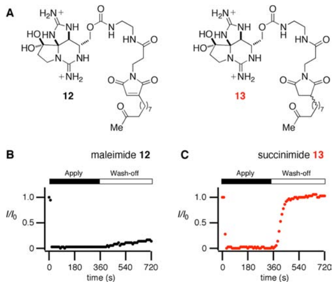
Figure 4. (A) Structures of C2-substituted maleimide ( 12 ) and succinimide ( 13 ) derivatives of STX. (B) Representative time course of wash-off of 5 \mu\text{M} 12 from CHO cells expressing \text{rNa}_v1.2 . (C) Representative time course of wash-off of 5 \mu\text{M} 13 from CHO cells expressing \text{rNa}_v1.2 . Average current recovery after washout was 22 \pm 5\% of I_0 for 12 , compared to 106 \pm 6\% for 13 . Data represent the average of 3–5 cells \pm SEM.
