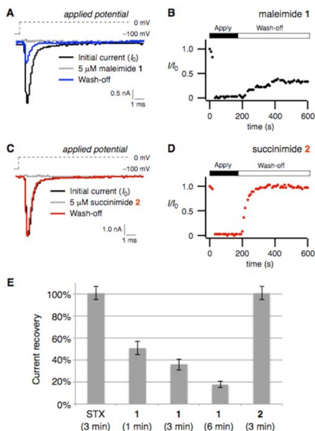
Figure 1. (A) Current recordings, elicited by a 10 ms voltage step from -100 to 0 mV, upon 3 min application and wash-off of 5 \mu\text{M} maleimide 1 to CHO cells expressing rNa v 1.4. (B) Representative wash-off time course for 1. (C) Current recordings upon 3 min application and wash-off of 5 \mu\text{M} succinimide 2. (D) Representative wash-off time course for 2. Average current recovery after washout was 36 \pm 5\% of I_0 for 1, compared to 101 \pm 6\% for 2. Data represent the average of 3–5 cells \pm SEM. (E) Current recovery following 8 min washout (incubation time for each compound shown in parentheses). Data represent the average of 3–7 cells \pm SEM.
