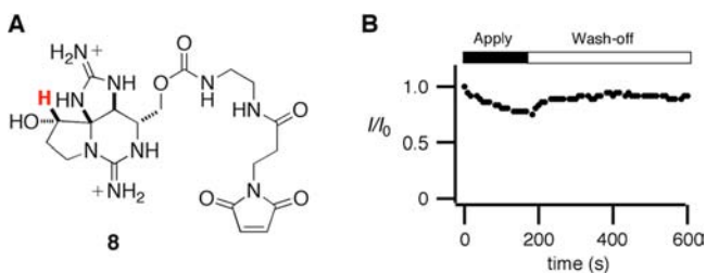
Figure 3. (A) Structure of maleimide-conjugated \beta -saxitoxin 8 . (B) Representative time course of wash-off of 5 \mu\text{M} 8 from CHO cells expressing \text{Na}_v1.4 . Current recovery after washout was 94 \pm 7\% of I_0 , which represents the average of 5 cells \pm SEM.
